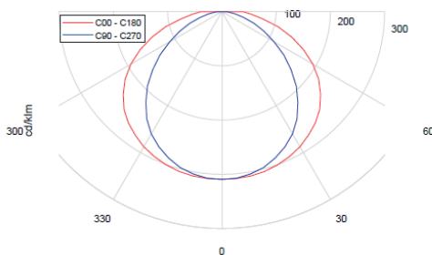
light distribution
